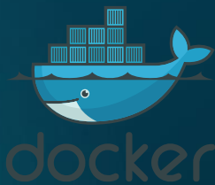
Docker
